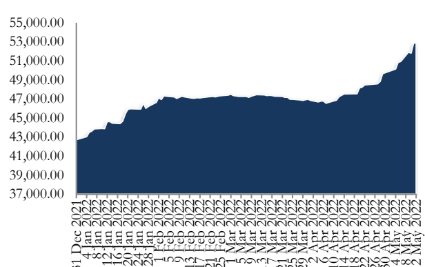
Fig. 3: NGX-ASI (Year-to-Date)
