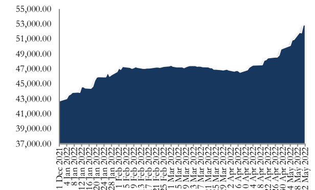
Fig. 3: NGX-ASI (Year-to-Date)
