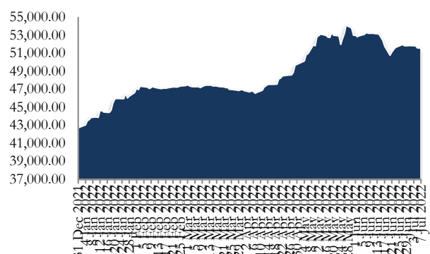
Fig. 3: NGX-ASI (Year-to-Date)
