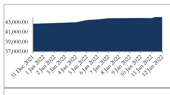
Fig. 1: NGX-ASI (Year-to-Date)
