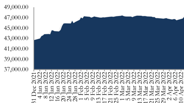
Fig. 3: NGX-ASI (Year-to-Date)
