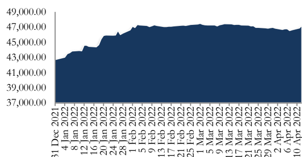
Fig. 3: NGX-ASI (Year-to-Date)
